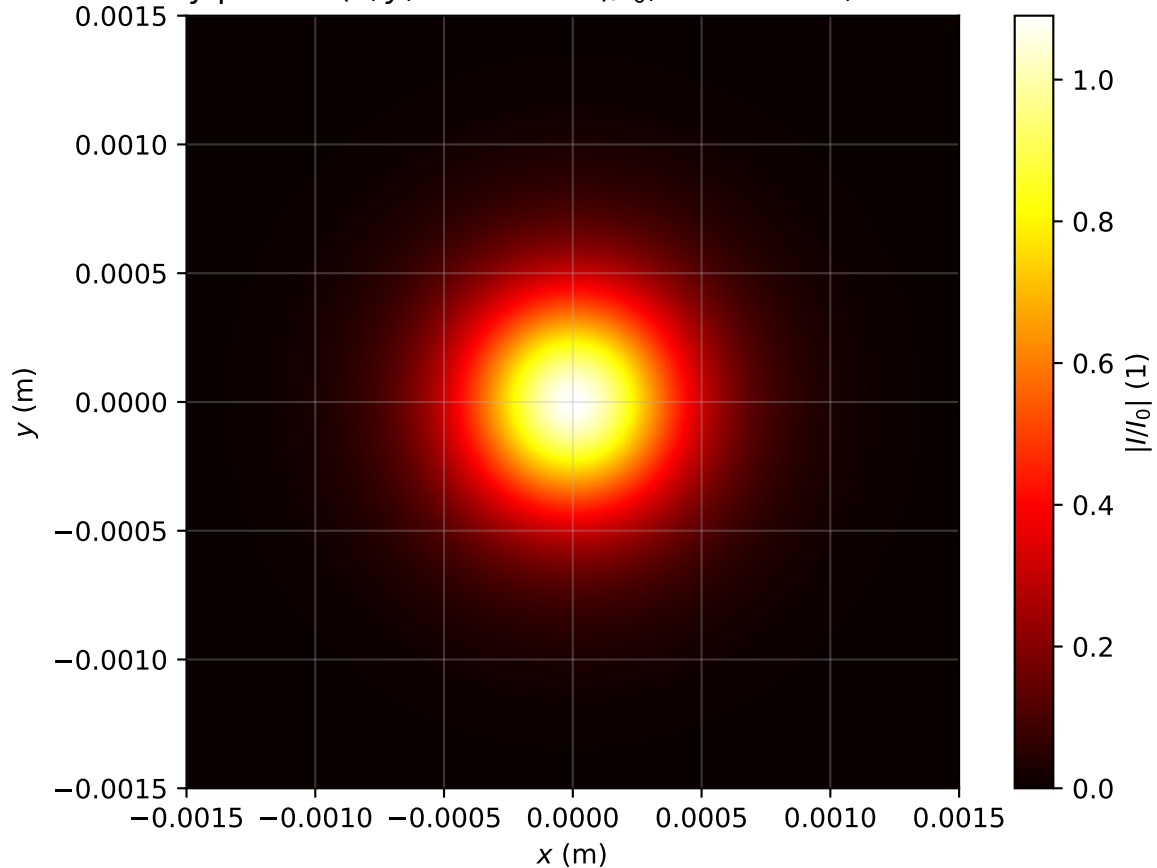
Intensity profile I(x, y, z = 1.353m)/I_0 , P_{in}=0.6P_{cr} , artificial time
